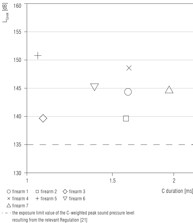
Figure 2. A list of C duration and C-weighted peak sound pressure level ( L_{Cpeak} ) values that characterize impulse noise generated during shots from the various types of firearms included in the tests
